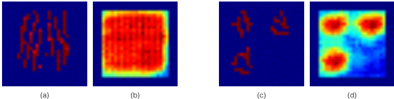
Figure 3: (a) Constant grid pattern observed in the attention masks on Translated MNIST. (b) Accuracy of the pre-trained classifier on 7 \times 7 digits centered at different pixels. Each pixel in the images is colored according to the estimated normalized accuracy on digits centered at that pixel where warmer colors indicate higher normalized accuracy. Only pixels that correspond to a possible digit center are represented in these images, with other pixels colored dark blue. (c–d) Duplicate of (a) and (b) for a pre-trained network on a modified Translated MNIST domain where no digits can appear in the bottom right hand corner.
